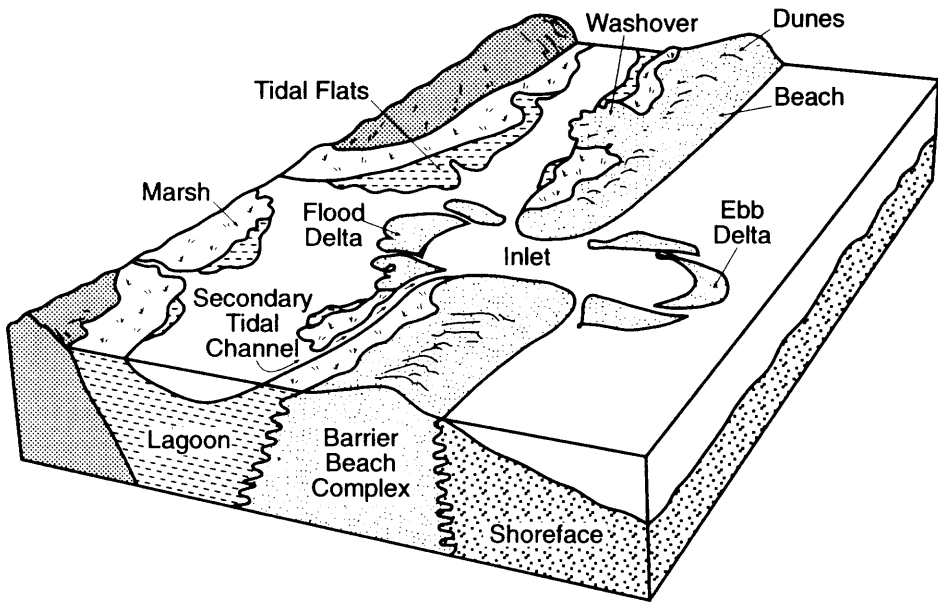
Figure MDe-10. Subdivision of a typical modern barrier island system and its environments. Modified from Reinson (1984).
