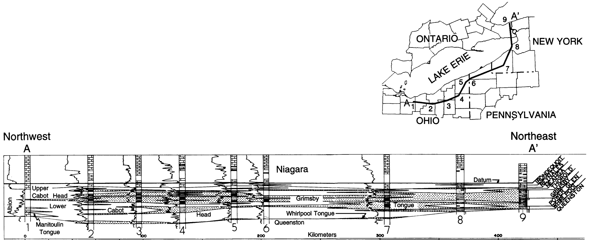
Figure Scm-4. Regional stratigraphic strike cross section A-A' of the Cataract/Medina Group interval. Modified from Knight (1969). Nomenclature is that of Knight (1969). (McCormac and others, 1996)
