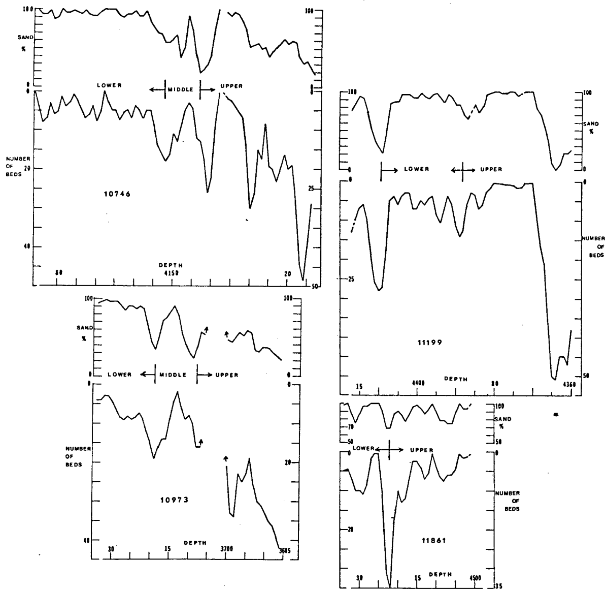
FIG. 34 PLOT SHOWING NEGATIVE CORRELATION BETWEEN SAND PERCENT &amp; NUMBER OF BEDS IN THE BENSON CORES.
