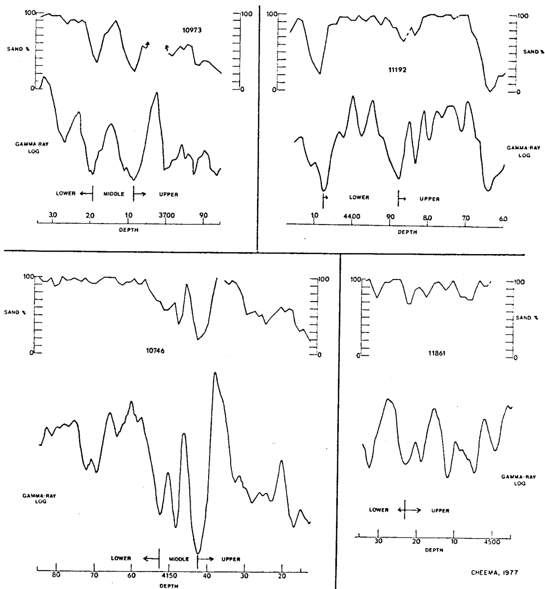
4700100396 FIG. 4 PLOT SHOWING CLOSE CORRESPONDENCE BETWEEN GAMMA-RAY LOG AND SAND PERCENT IN THE BENSON CORES
