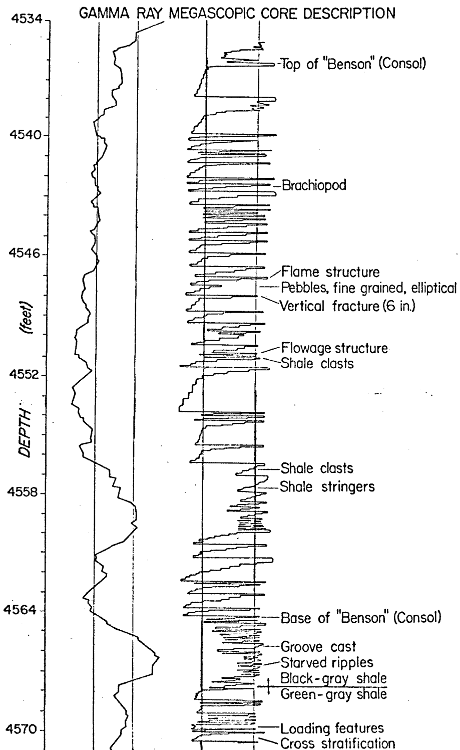
FIG. 3 COMPARISON OF LOG AND CORE DATA (CONSOL I1889)
